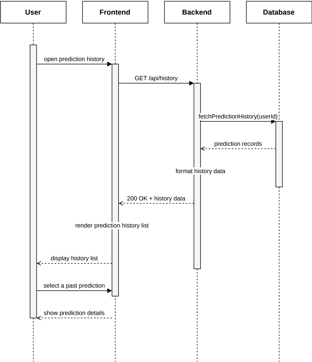
Sequence Diagram — View Prediction History
